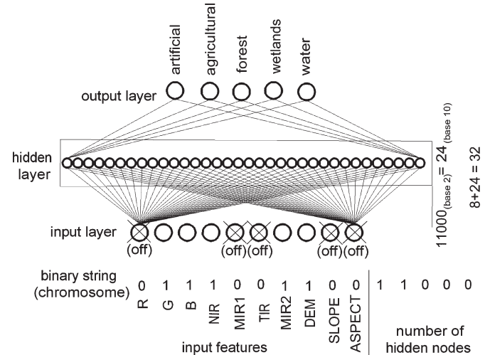
Fig. 1. Genetic-algorithm representation and mapping on to a corresponding neural network. The network is fully connected, but note all the connections are shown here. Zero values in the string denote inactive input nodes (OFF). The number of hidden nodes is the sum of the constant eight plus the five-bit binary number converted to decimal.
