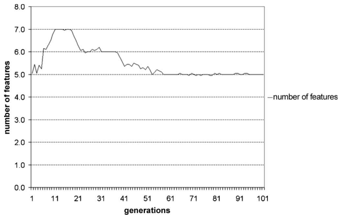
Fig. 4. Average number of features per generation during optimization with the genetic algorithm.
