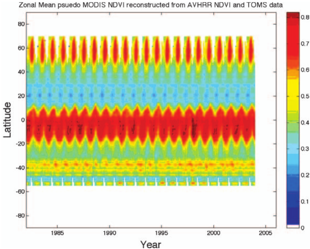
Figure 4. Latitude-averaged mean of NNndvi from 1982 to 2003.
